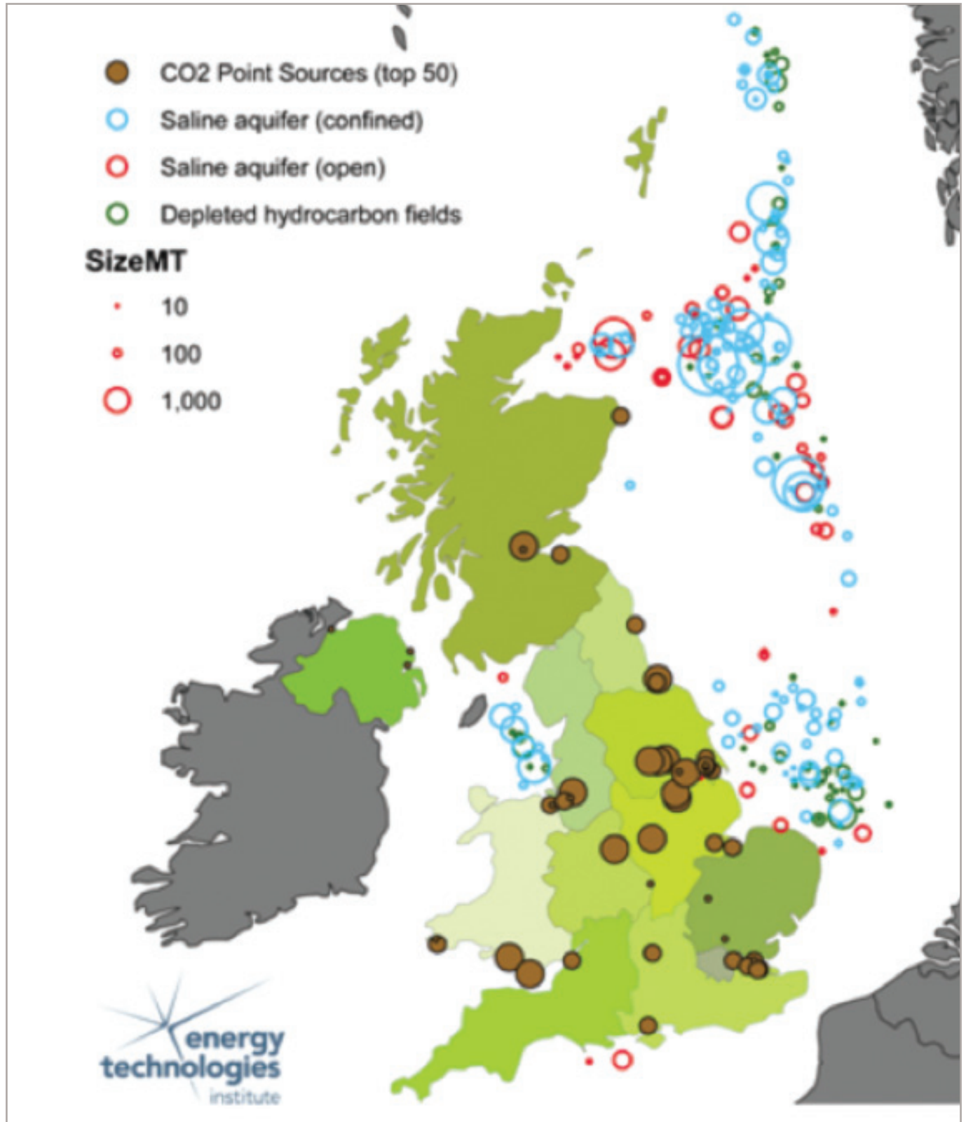
Figure 2. Proximity of the UK's largest industrial emitters to CO 2 storage sites in the North and Irish Seas xxv
